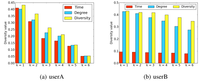
Figure 7: Query: privacy: Diversity analysis
