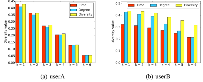
Figure 6: Query: budget: Diversity analysis
